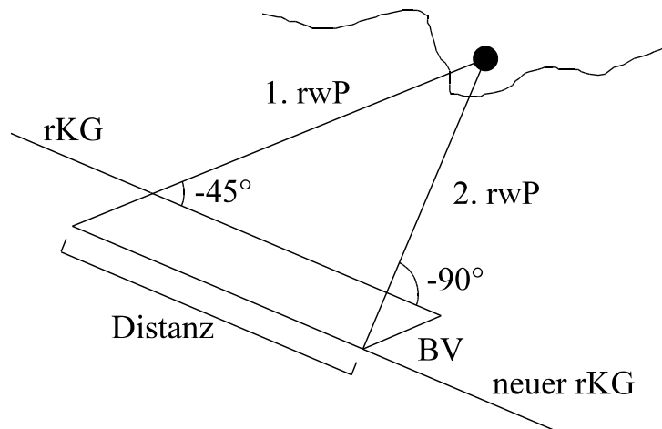
Abb. 18: 4-Strich-Peilung
